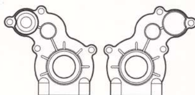
P7126 Transmission Carrier 变速箱壳 2pc
