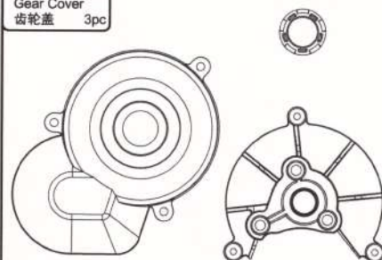
P7127 Gear Cover 齿轮盖 3pc
