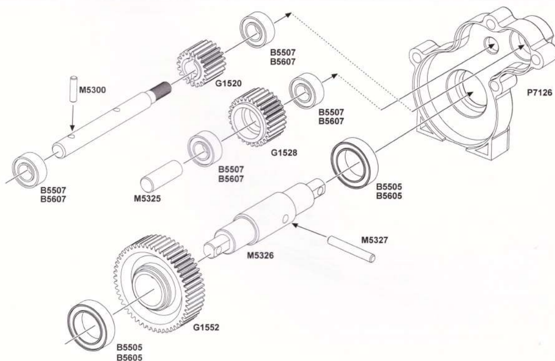
B5602/B5605/B5607 为粉末铜套 powder-sintering copper sleeve
